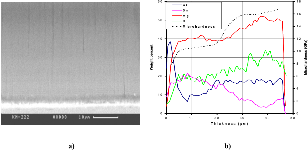
Figure 3: Microstructure (a) and distribution of chemical elements and variation of microhardness value along the sample cross-section in the coating cross-section (b).
