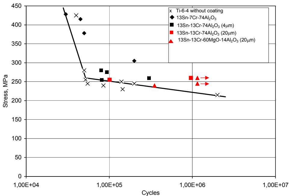
Figure 6: Dependence of the number of flat sample vibrations up to their fracture on the magnitude of deformation amplitude.
